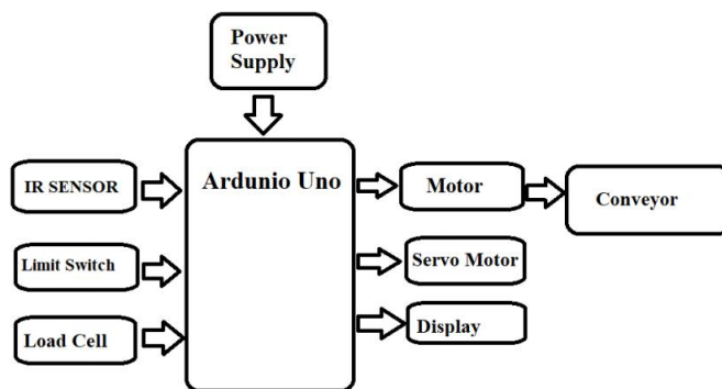
Figure 1: Block Diagram
