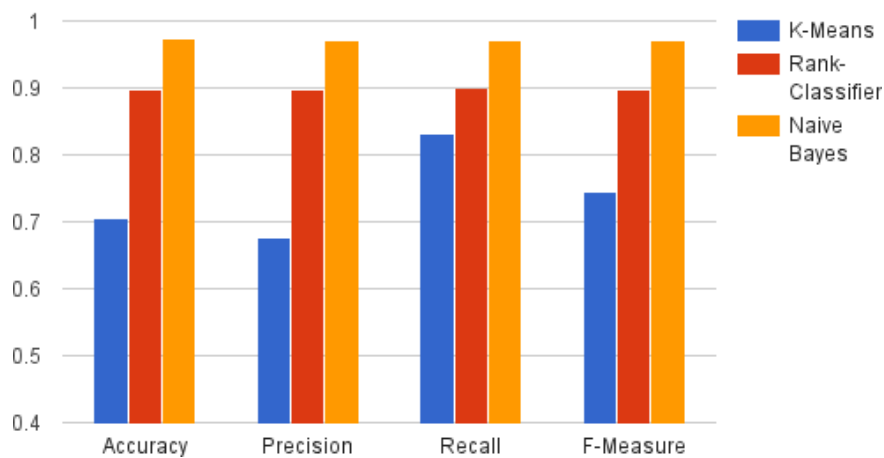
Figure 1: Classifier Performance Comparison.
