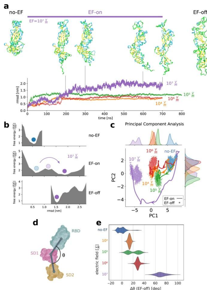
Fig.13 Electric fields are able to induce global conformational changes in the spike glycoprotein SP, affecting the stability of folding states. a, b EF driven major shape changes occur in the different subunits and between subunits of the S protein.
