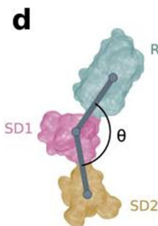
Fig. n. 24 Field-induced conformational states can be characterised by the angles formed by the vectors connecting the centroids of clustered residues. from doi: 10.1038/s41467-021-25478-7
