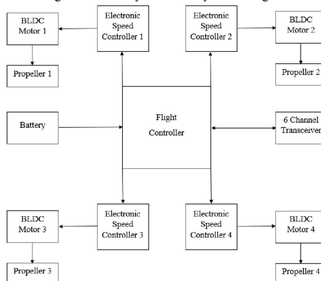
Figure 2. Drone Body block diagram
