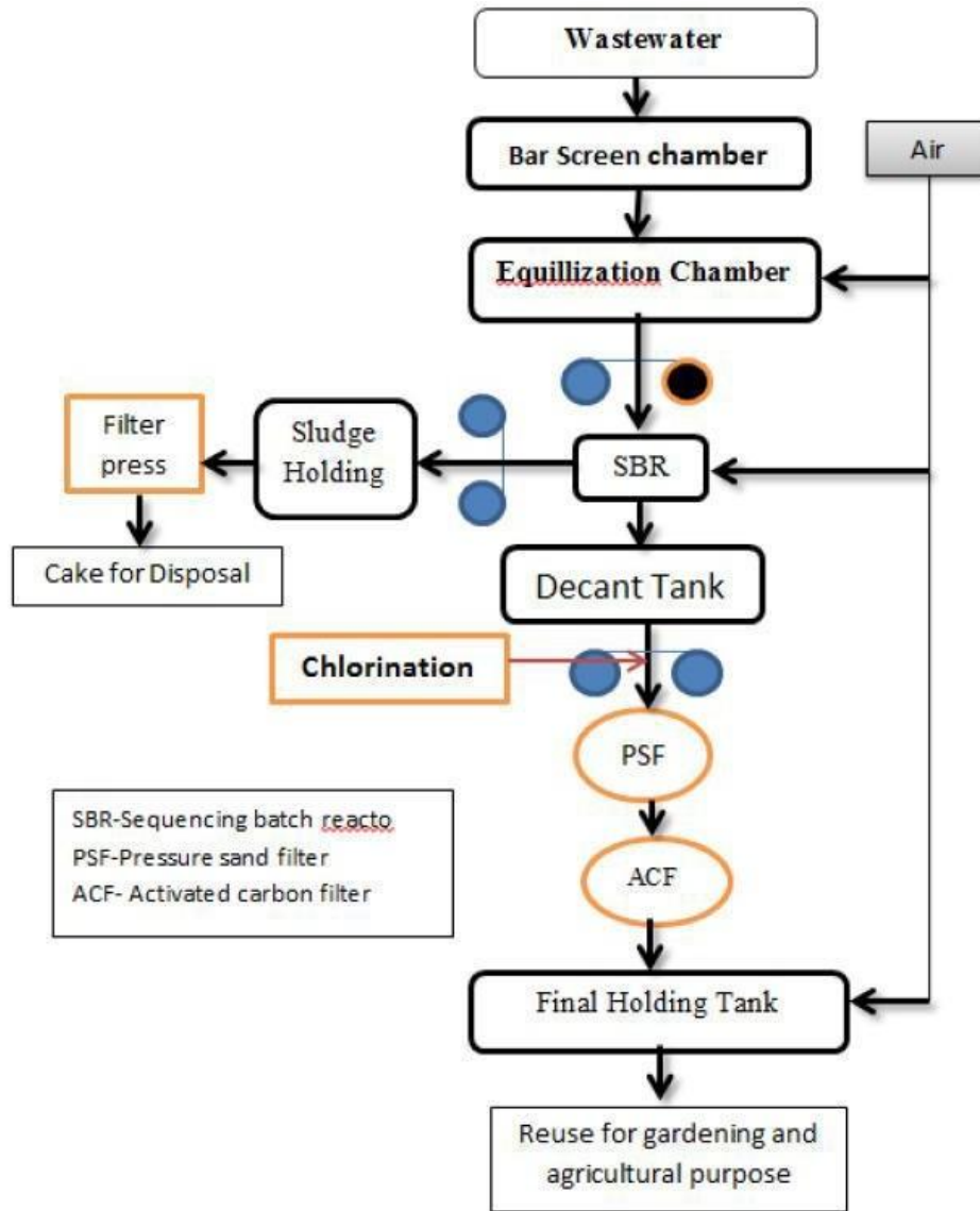
Figure: SBR Flow Diagram
