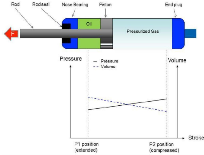
Fig. 2 Gas Spring schematic - Pressure/ Volume vs. stroke diagram. As the piston moves from the fully extended position (P1) to the fully compressed position (P2), the pressure (solid line) rises and the volume (dashed line) reduces.
