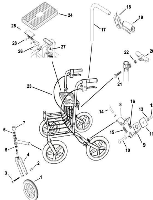
Fig. 1 Rollator Parts
