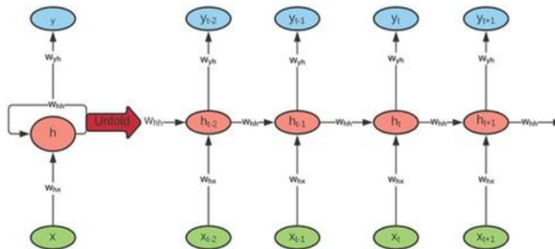
Figure 1. Recurrent neural network cell structure.
