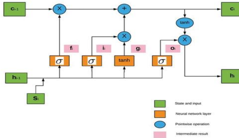
Figure 2. Long short-term memory cell
