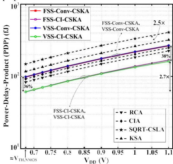
Figure 12: Energy–delay Pareto-optimal curves for different adders
