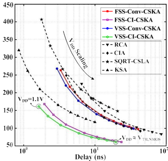
Figure 10: PDP of the adders versus the supply voltage.
