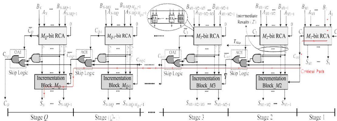
Figure 2: Proposed CI-CSKA structure.
