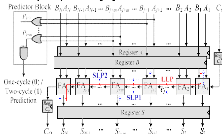
Figure 5: Generic structure of variable latency adders based on RCA.
