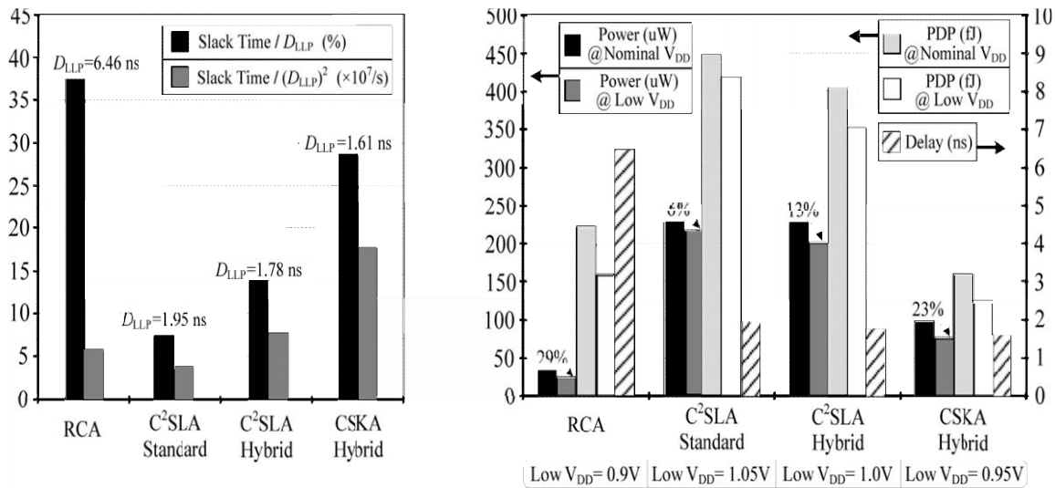
Figure 14: (a) Ratio of the slack time to DLLP, and the ratio of the slack time to (DLLP) 2 for the four studied variable latency adders. (b) Power consumption and PDP at the nominal and low VDD for the adders. (Nominal VDD is 1.1 V for all the structures.)
