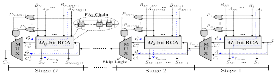
Figure 1: Conventional structure of the CSKA [19]
