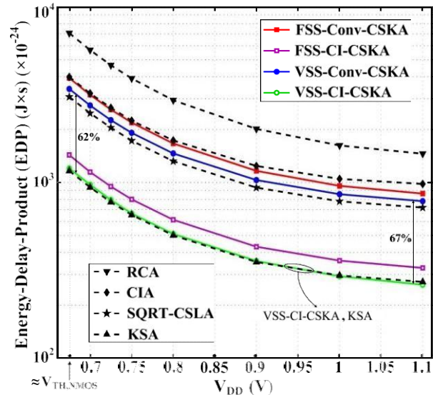
Figure 11: EDP of the adders versus the supply voltage.
