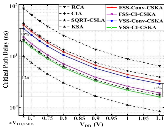
Figure 8: Critical path delay of the adders versus the supply voltage.
