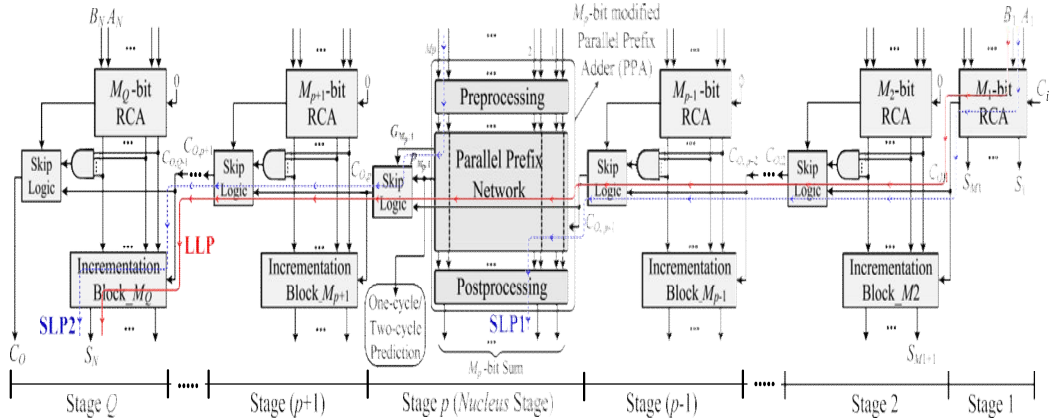
Figure 6: Structure of the proposed hybrid variable latency CSKA.
