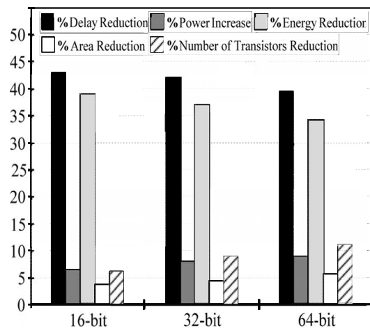
Figure 13: Changes of delay, power, energy, area, and number of transistors
