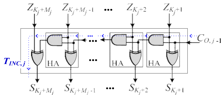
Figure 3: Internal structure of the j th incrementation block,
