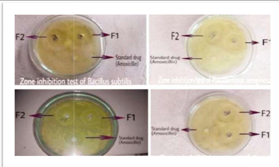
Plates showing zone of inhibition for different organism
