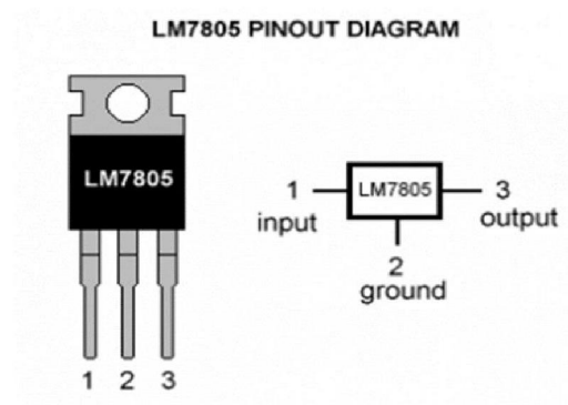
Fig 10 : LM7805 Pinout Diagram
