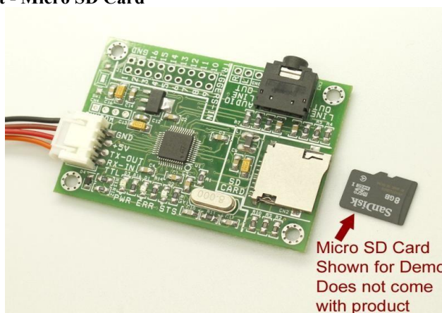
Fig 3: audio Player
