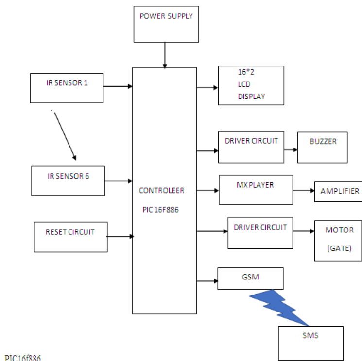
Fig 1: Block Diagram
