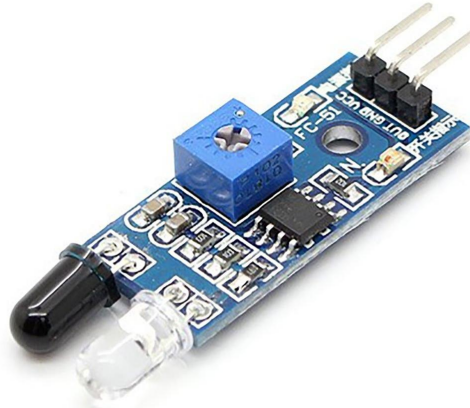
Figure 4.3: IR Sensor
