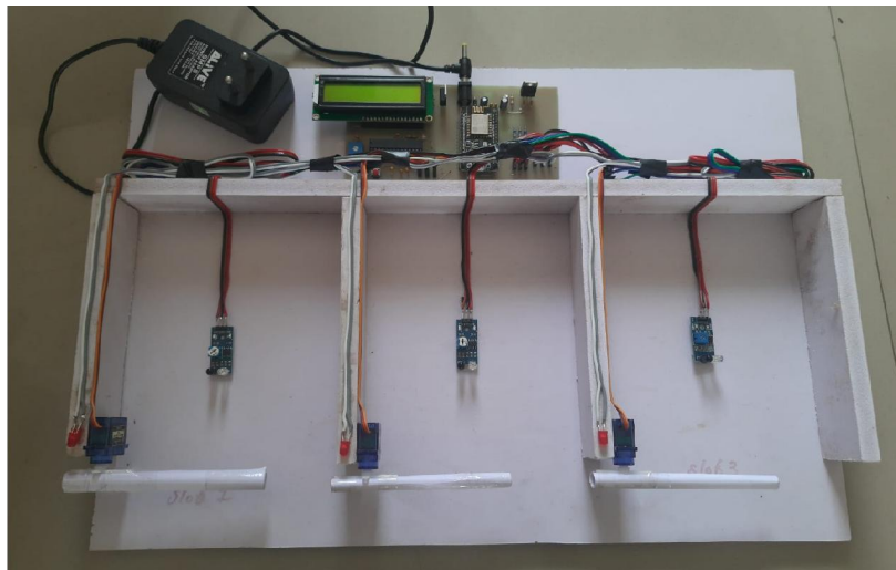
Figure 7.1: Admega 238 and Node MCU
