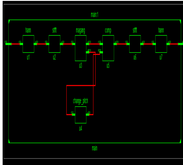
Figure 5.2: RTL of Phase Vocoder
