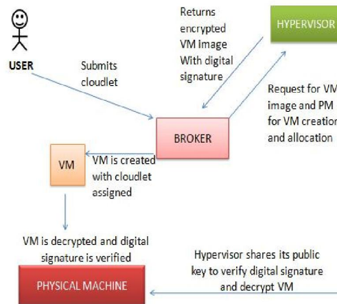
Fig 5.2: Attack on VM image through malicious activity by cloudlet
