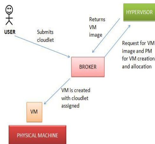
Fig 5.1: Figure showing VM image sharing concept in cloud
