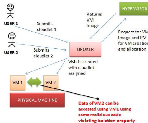
Fig 5.3: Figure showing data theft by VM1 on data of VM2
