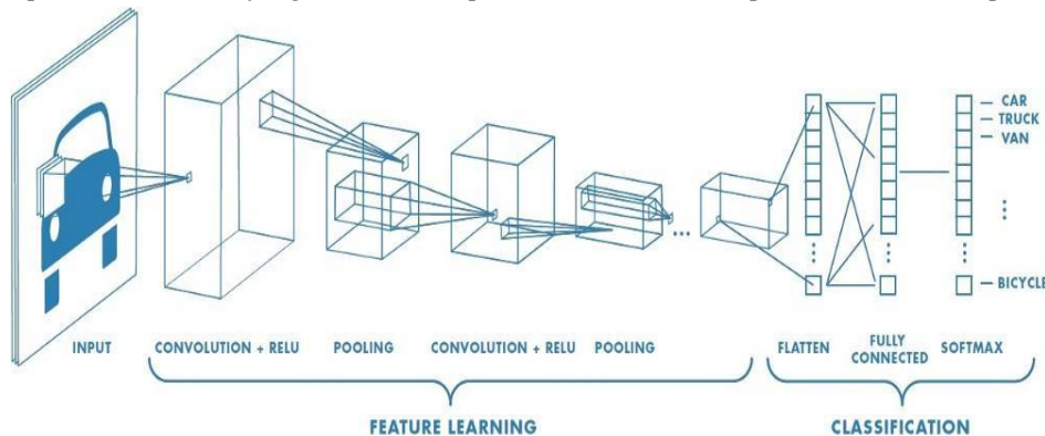
Fig. 5. LeNet-5 structure in modelling CNN for a 28x28 input image
