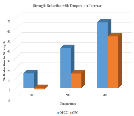
Figure 4: Graphical Representation of Strength Reduction with Temperature
