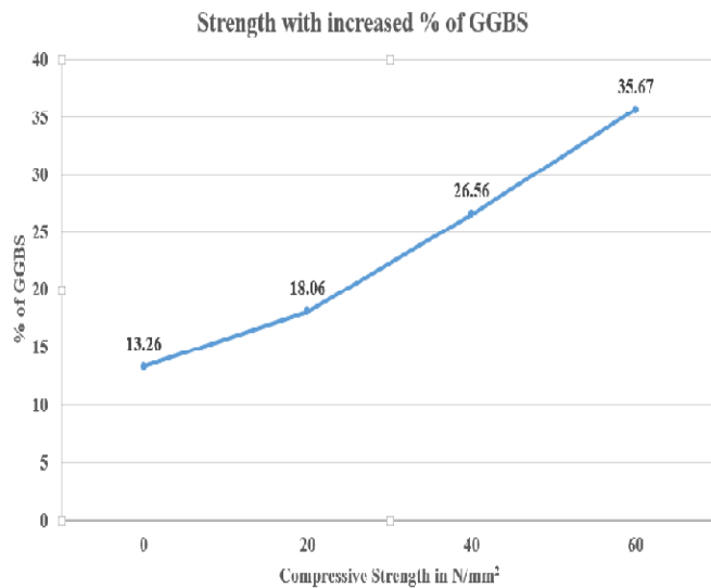
Figure 1: Graphical Representation of strength variation with increase in % of GGBS
