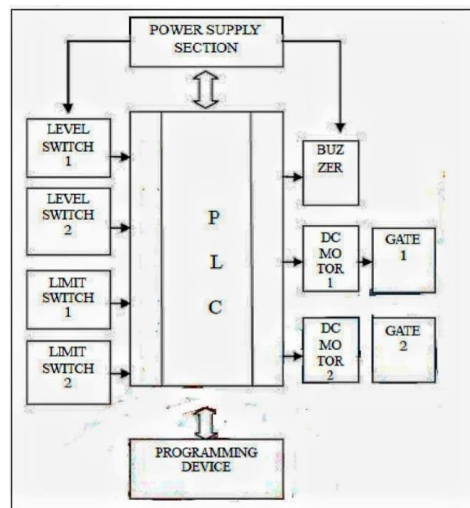
Figure 1: Block diagram of system using PLC
