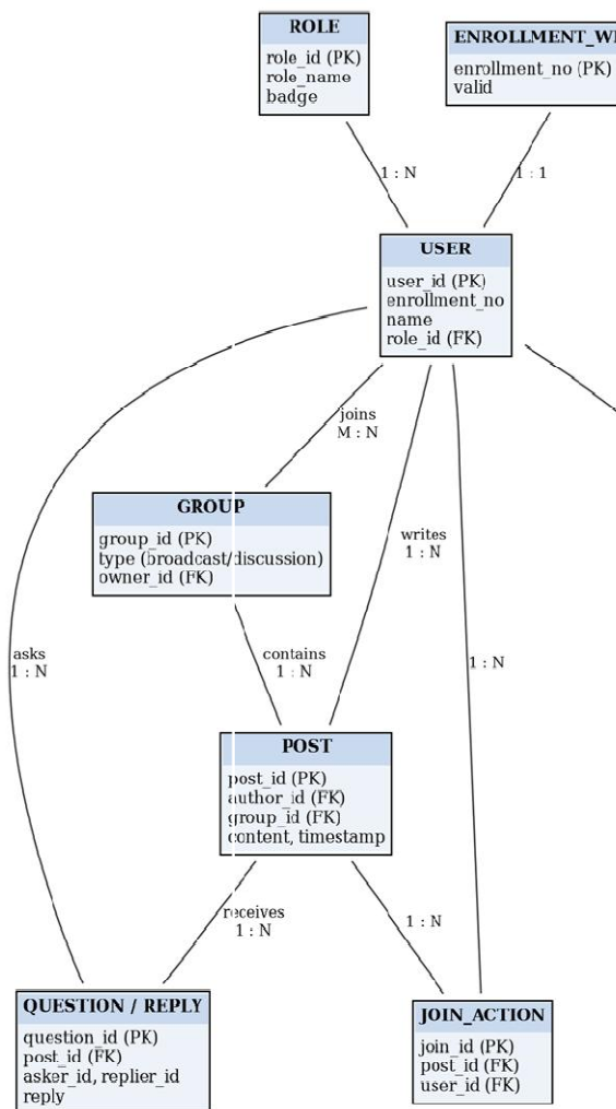
Fig. 3. Entity-relationship diagram
