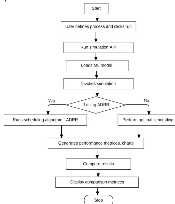
Fig. 1: Flowchart of Proposed ADRR Scheduling Frame-work
