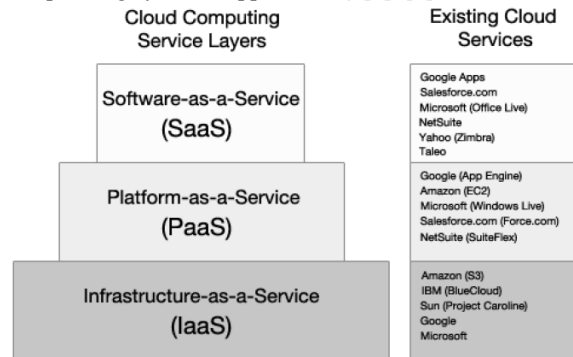
Figure 3.1: Showing the Cloud Computing Stack and Existing Cloud Services [20].
