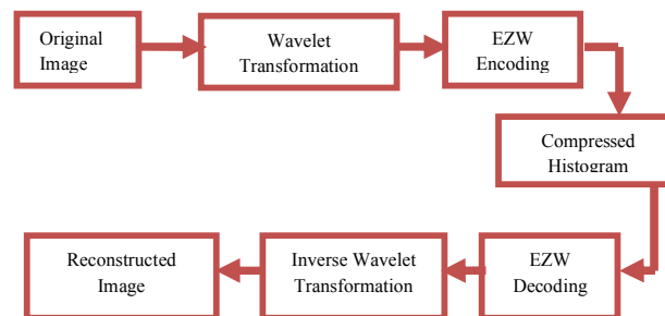
Fig 1. Flow Chart of EZW Decoding [9]
