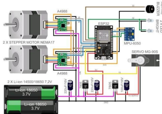
Fig.1 Connection
