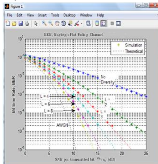
Figure 3: BER, Rayleigh Flat Fading Channel.
