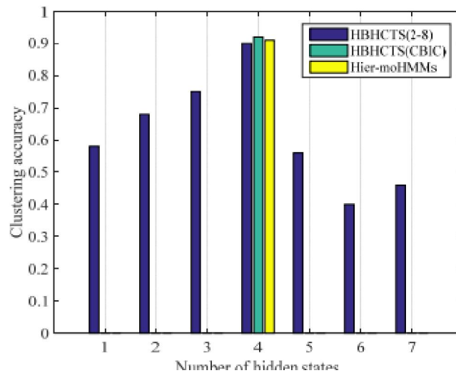
FIGURE 7. Corrected-rate of different clustering methods on the synthesized data.
