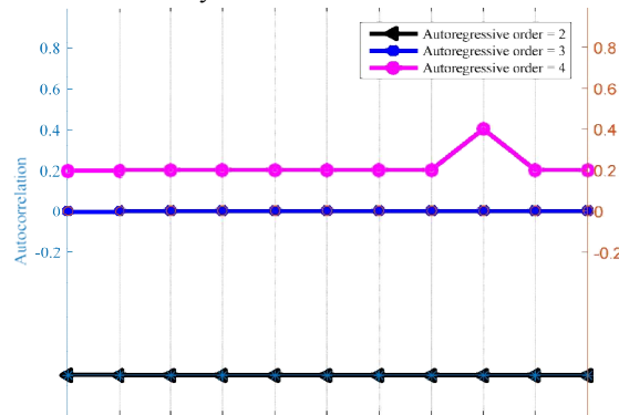
FIGURE 10. Autocorrelation diagram of time series
