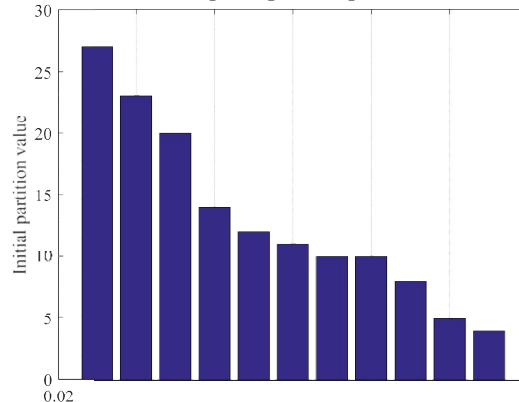
FIGURE 9. Number of initial partitions at different distance thresholds.
