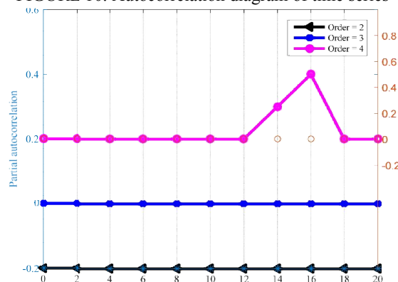
FIGURE 11. Partial autocorrelation diagram of time series
