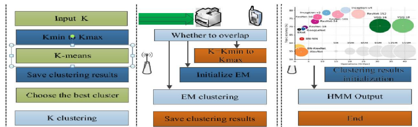
FIGURE 9. HBHCTS_algorithm_flowchart.
