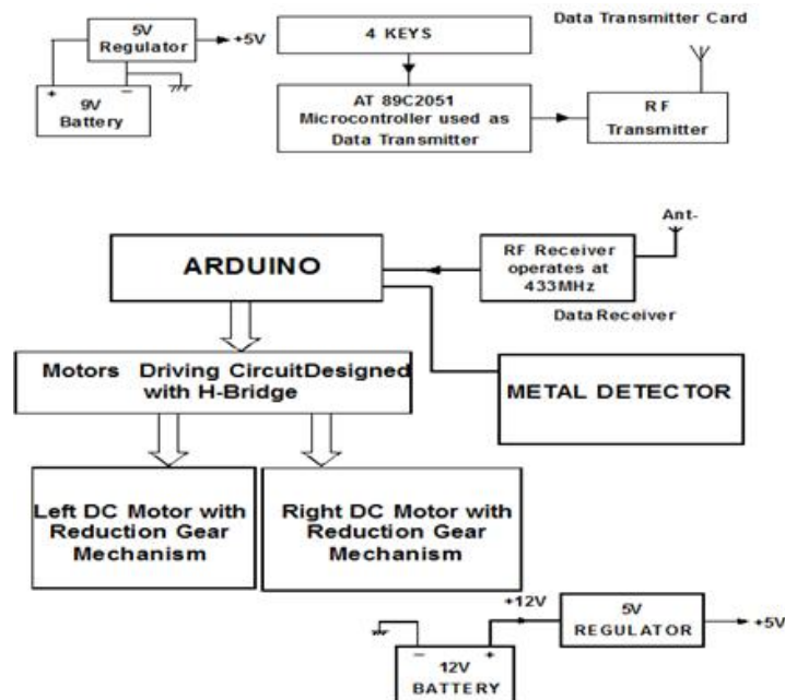
Figure 2: Block diagram of Hardware
