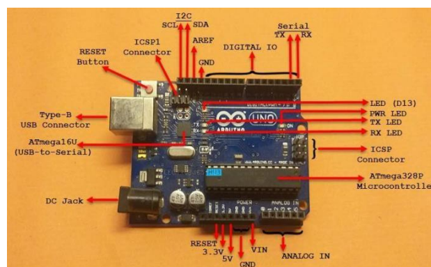
Figure 1: Arduino Uno Hardware
