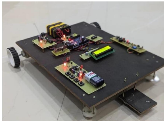
Figure 3: METAL DETECTOR ROBOT
