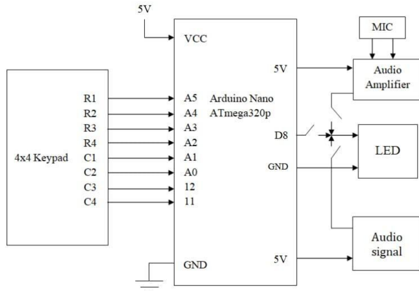
Fig 1:- Transmitter Interfacing Diagram
