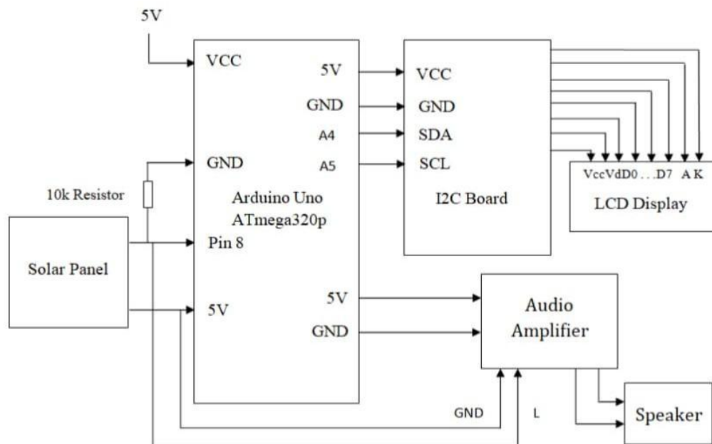
Fig 2:- Receiver Interfacing Diagram
