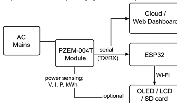
Fig. Smart Energy Meter with load
