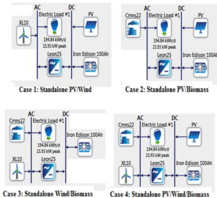
Fig. 1: Different stand-alone configurations in HOMER.
