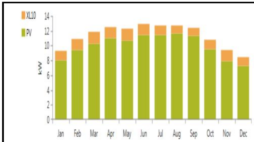
Fig. 3: The monthly average electric output of case 1.
