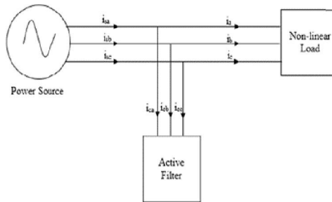
Figure 3.1 Shunt active Power Filter
