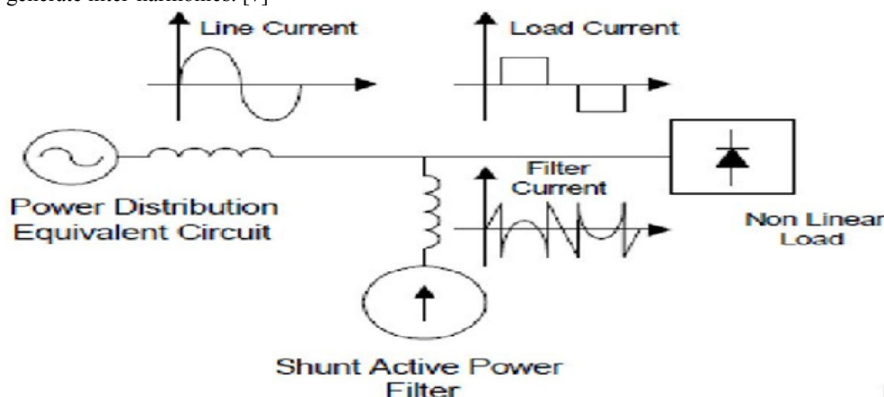
Figure 2.1 Power Quality Improvement
