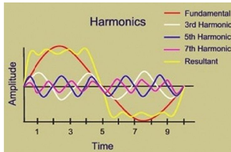
Figure 4.1 Harmonics in Power System
