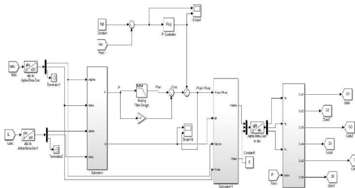
Figure 6.2 PQ theory control structure with PI controller of digital active power filter
