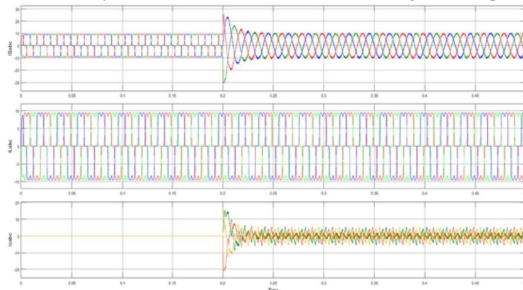
Figure 6.5 Source currents, Load currents and compensating current before and after digital active power filter
