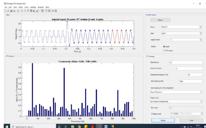
Figure 6.8 THD of source current with PI controller digital active power filter
