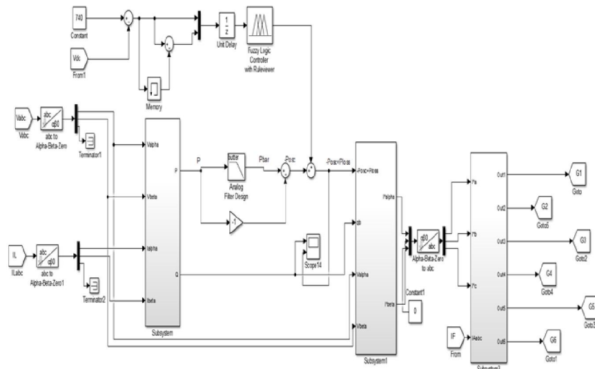
Figure 6.4 PQ theory control structure with FIS controller of digital active power filter
