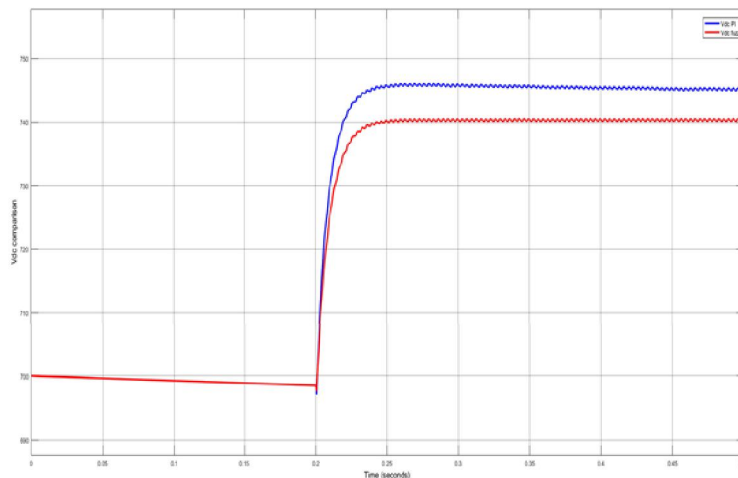
Figure 6.6 DC link voltage comparison at DC capacitor with PI and FIS controllers The above fig 6.6 is the DC link voltage comparison of PI and FIS controller of the PQ theory.
