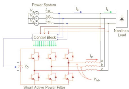
Figure 3.2 Shunt Active Power Filter Topology
