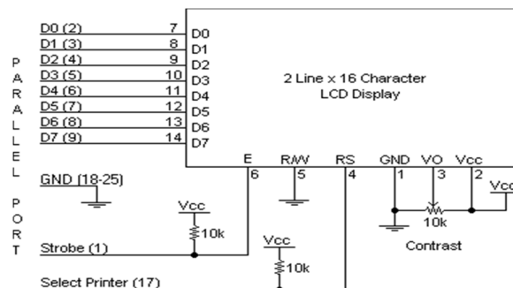
Figure 5: Circuit Diagram of the system
