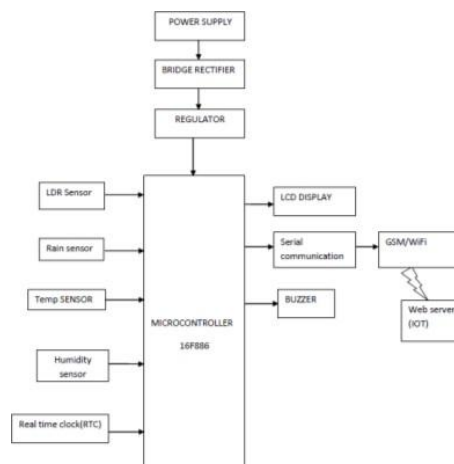
Figure 1: Block Diagram of the Project
