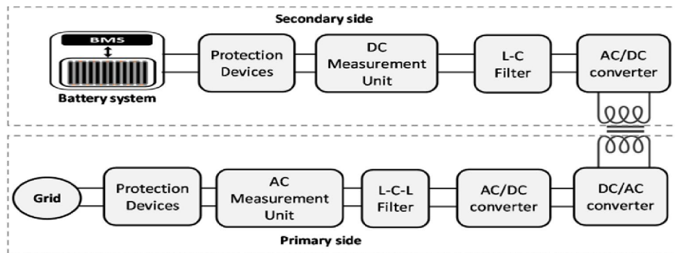
Figure 2. Example of the structure of an Inductive Charger.
