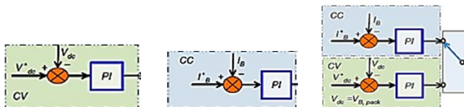
Figure 9. Charging methodologies control blocks and Voltage-Current Curves. (a) CV Charging; (b) CC Charging; (c) CC-CV Charging
