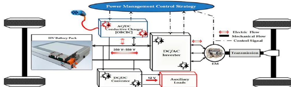
Figure 1. Diagram of the electric vehicle's components.
