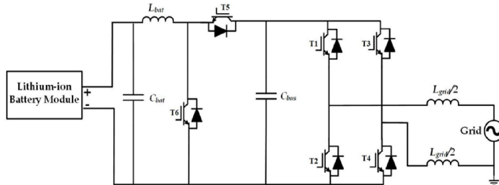
Figure 15. Simulink model of the FB and the Two-Quadrant converter for Light-Duty Vehicles.
