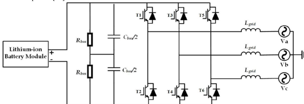
Figure 16. Simulink model of the FB for Heavy-Duty Vehicles.
