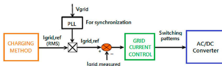
Figure 8. Main control blocks in the system.
