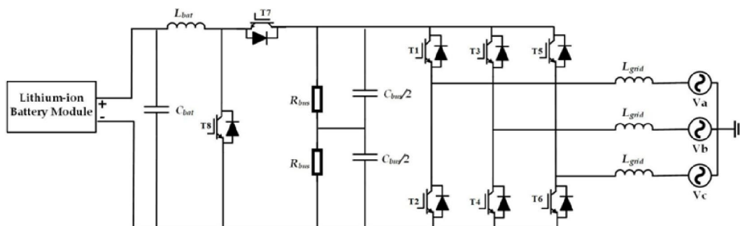
Figure 17. Simulink model of the FB and the Two-Quadrant converter for Heavy-Duty Vehicles.
