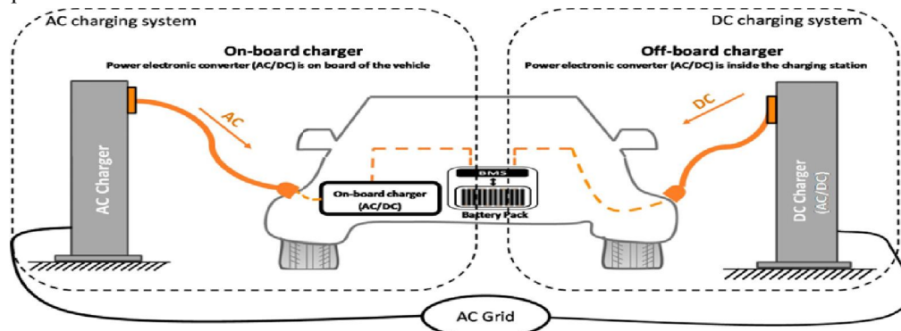
Figure 4. On-board charger versus off-board charger
