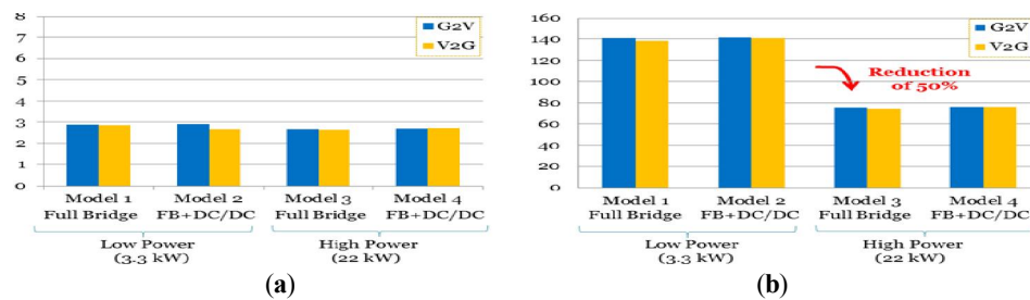
Figure 24. Total Harmonic Distortion of the AC waves in the four studied topologies. (a) Grid Current THD; (b) AC Voltage THD
