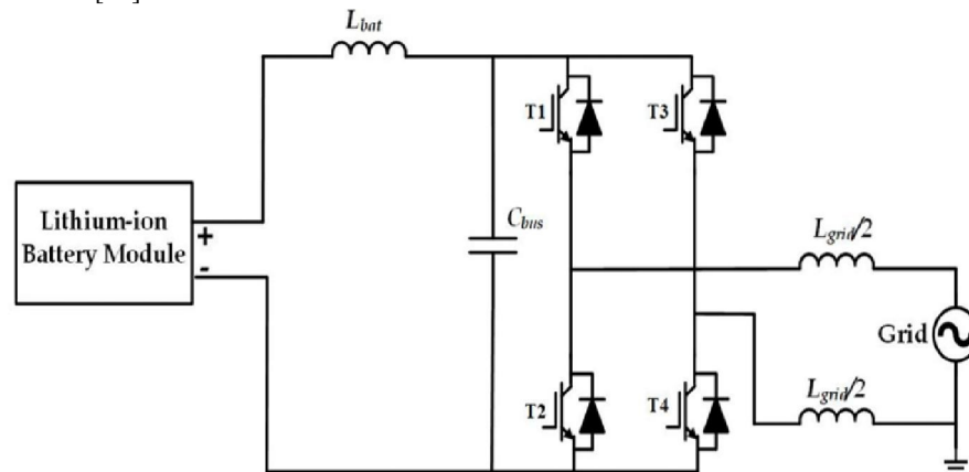
Figure 14. Simulink model of the FB for Light-Duty Vehicles
