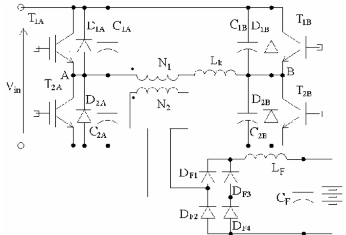
Figure 5: The H-bridge converter for charger
