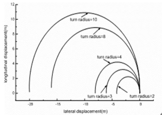
Figure 7: Locus of different turn radius achieved by skid steering
