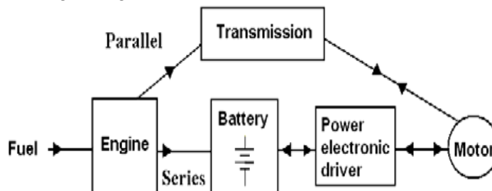
Figure 1: The series or parallel path of an HEV
