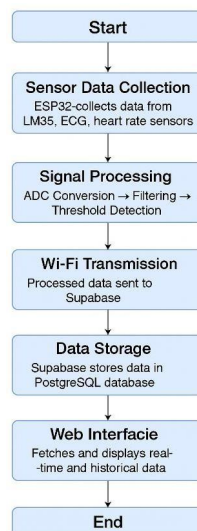
Fig 2.4 Flow Chart
