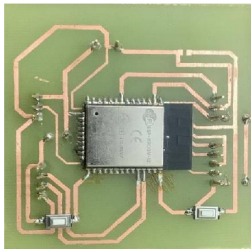
Fig. 2.2 Custom-Designed ESP32
