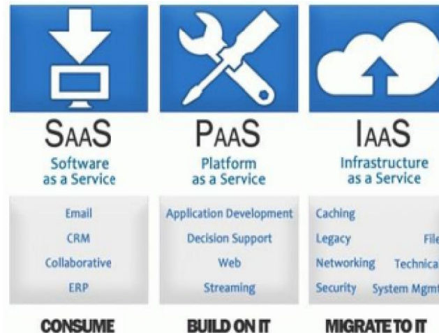
Fig.4 Cloud Services [8]
