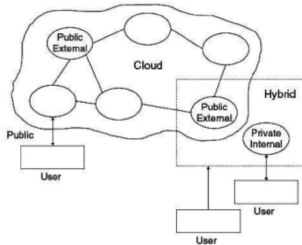
Fig.3 Cloud Models [3]
