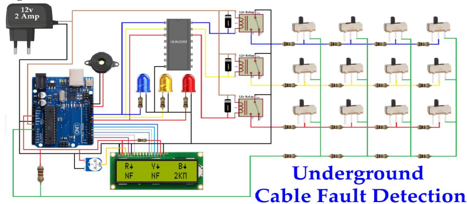
Fig.3 Circuit Diagram of System
