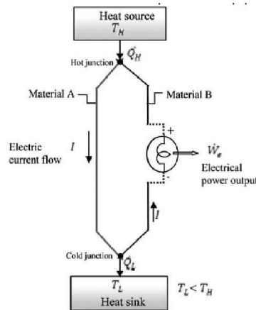
Fig.2. Working Principle
