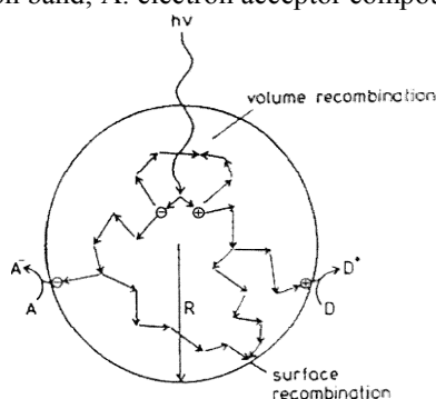
Figure 2: Fate of electrons and holes within a spherical particle of TiO 2 in the presence of acceptor A and donor D (Ollis et.al 1999).
