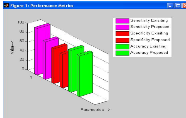
Fig.12 Performance Metrics
