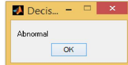
Fig.9 Decision
