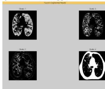
Fig.10 Segmented results
