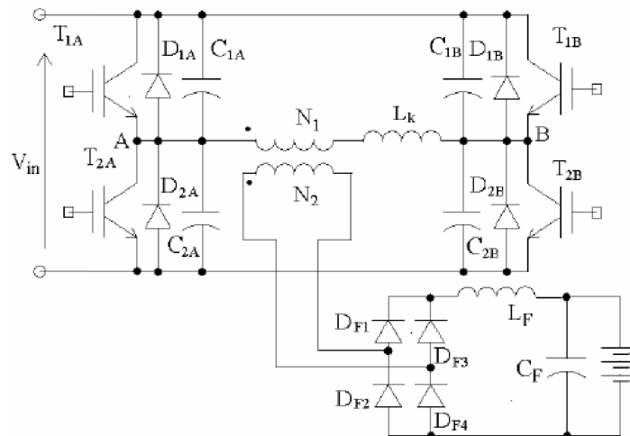
Figure 6: Schematic of the BMS
