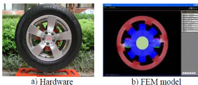
Figure 3: The in-wheel motor
