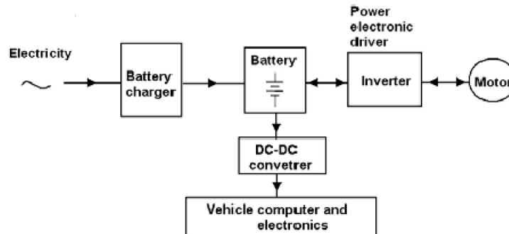
Figure 2: The key components of an Electric Vehicle.
