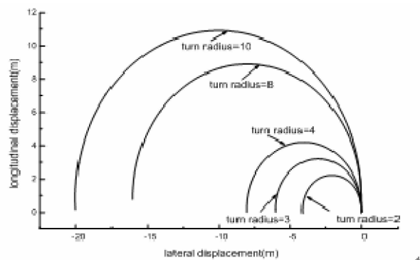
Figure 7: Locus of different turn radius achieved by skid steering
