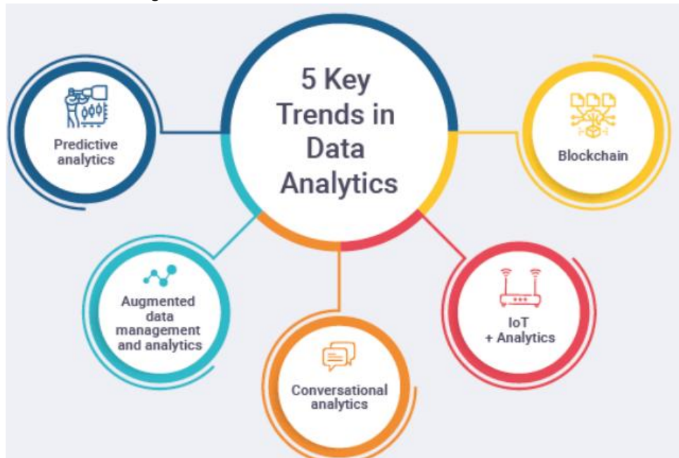
Figure 2: Data Analytics
