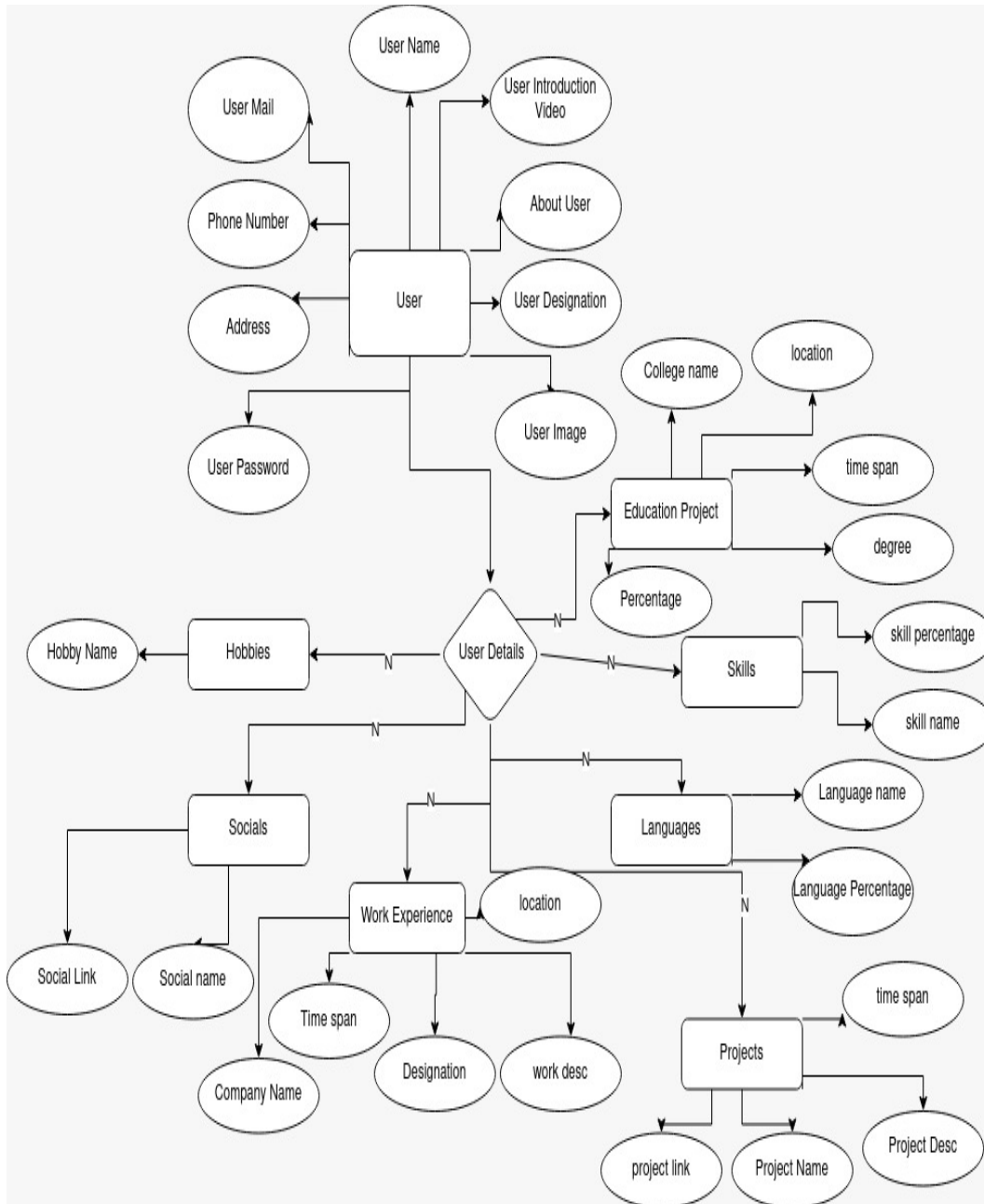
Fig 2: Entity Relationship Diagram
