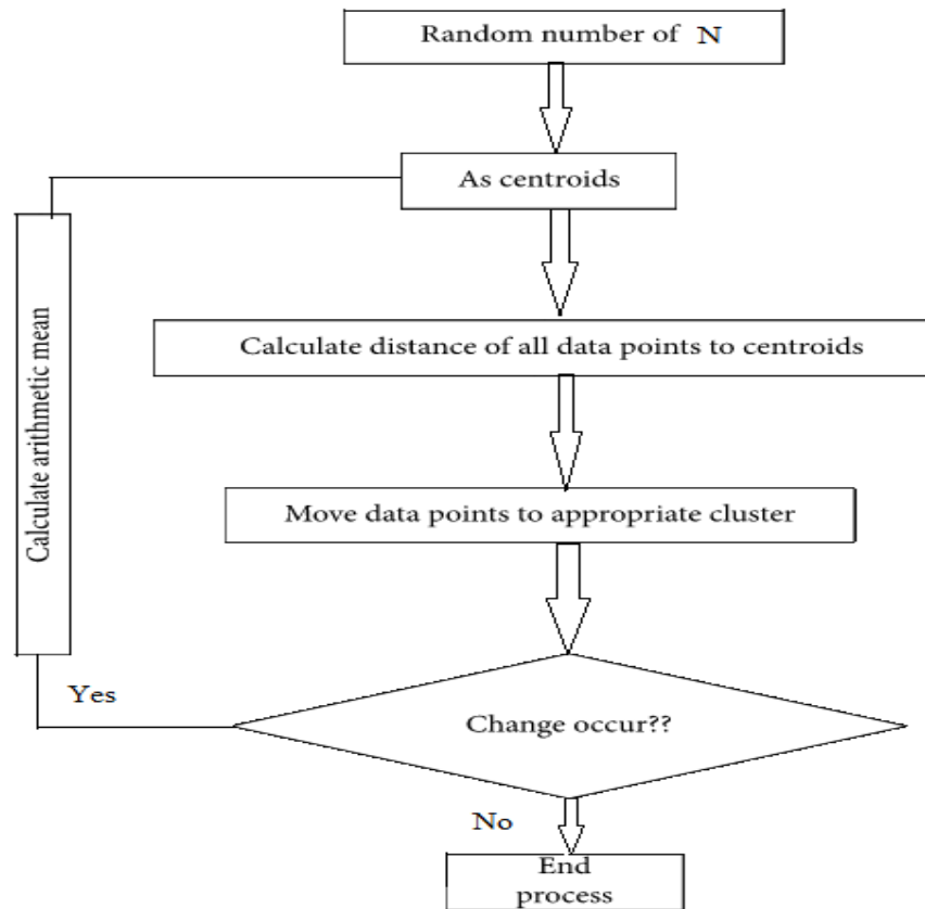
Fig. 2 Flowchart of CBKM
