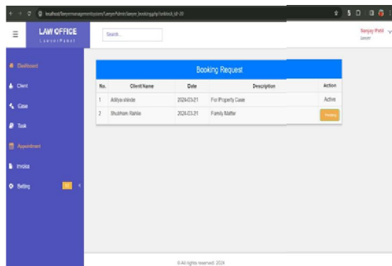
Fig 8 Booking Request
