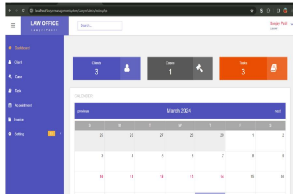
Fig 3 Admin_Lawyer_Active
