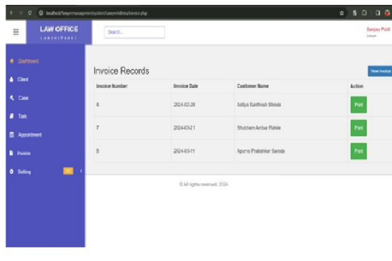
Fig 9 Invoice
