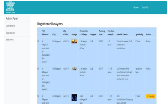
Fig 3 Admin_Lawyer_Active
