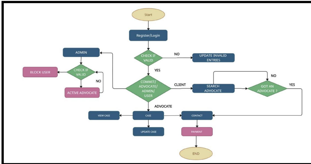
Fig.1 Flow Chart
