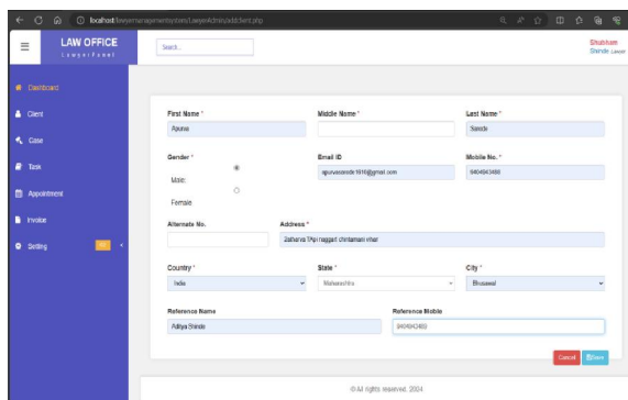
Fig 6 Add_Clients
