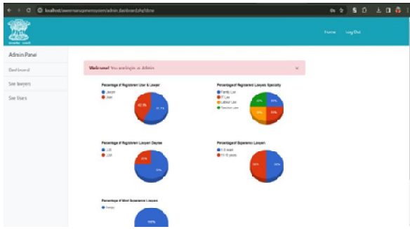
Fig 2 Admin_Panel
