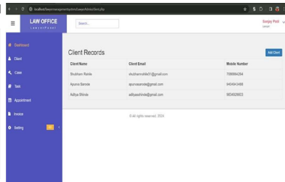
Fig 7 Client Records(Lawyer)
