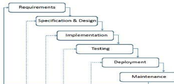
Figure 1.1: Waterfall Model
