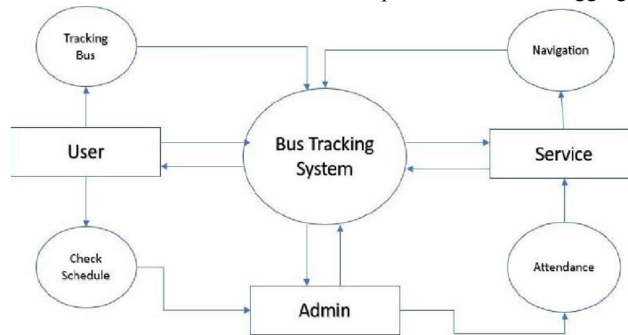
Figure 4.2: DFD Diagram
