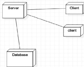
Figure 4.7: Deployment Diagram
