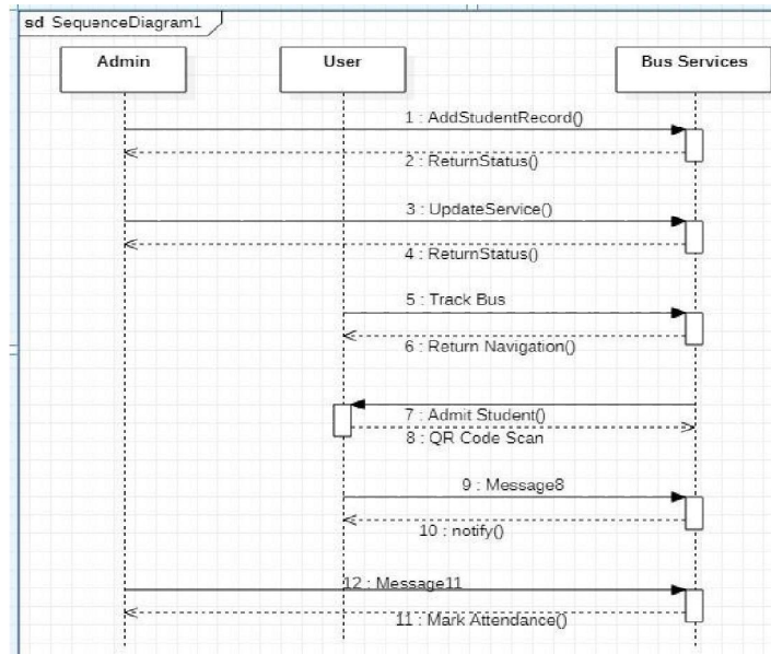
Figure 4.6: Sequence Diagram
