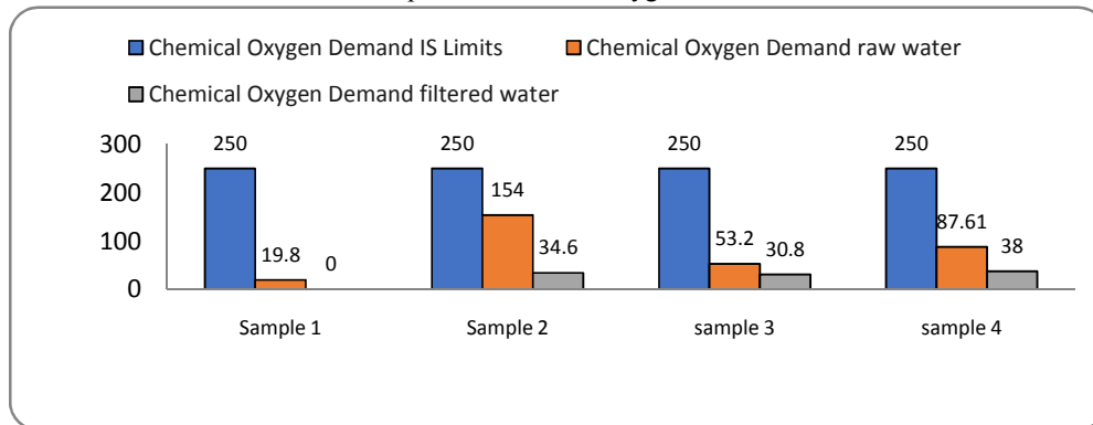
Graph 10. Chemical Oxygen Demand
