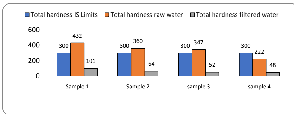
Graph 6. Total hardness
