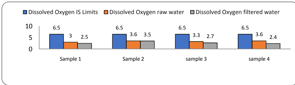
Graph 8. Dissolved Oxygen
