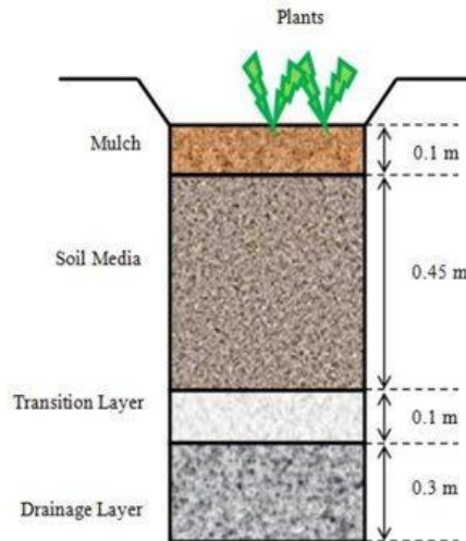
Fig 2.1 Bioretention System
