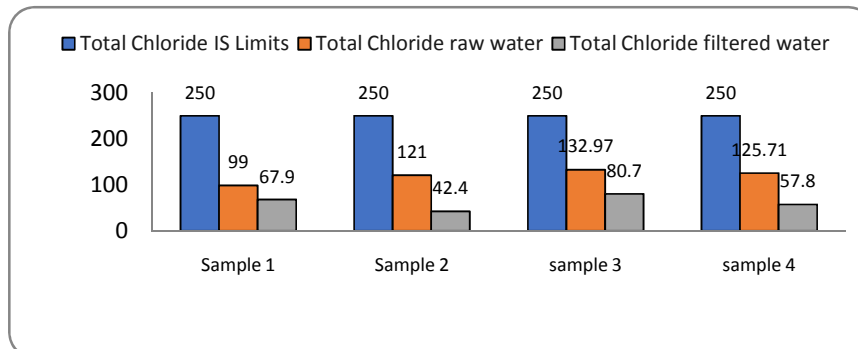
Graph 4. Total Chloride
