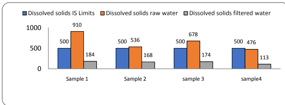
Graph 5. Dissolved Solids
