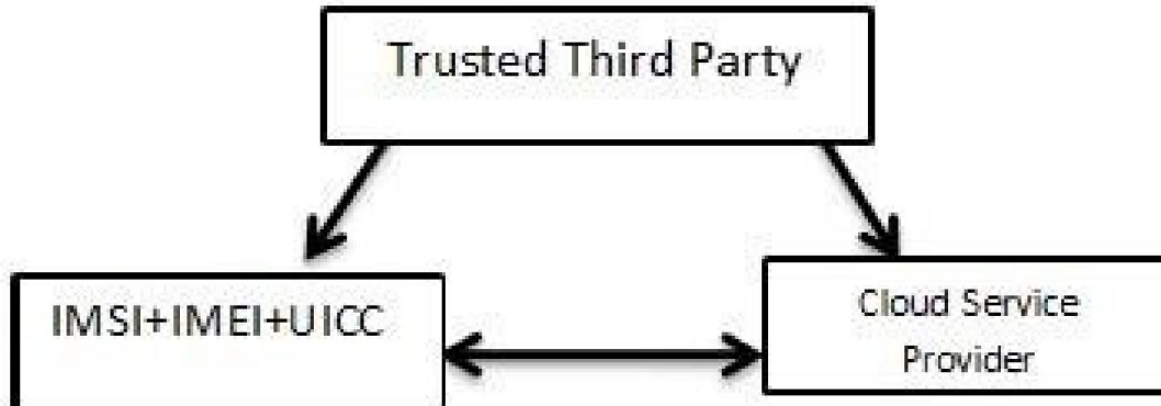
Fig. 2 Proposed Model
