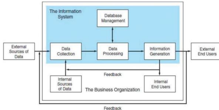
Fig. 1. Model of general accounting information system
