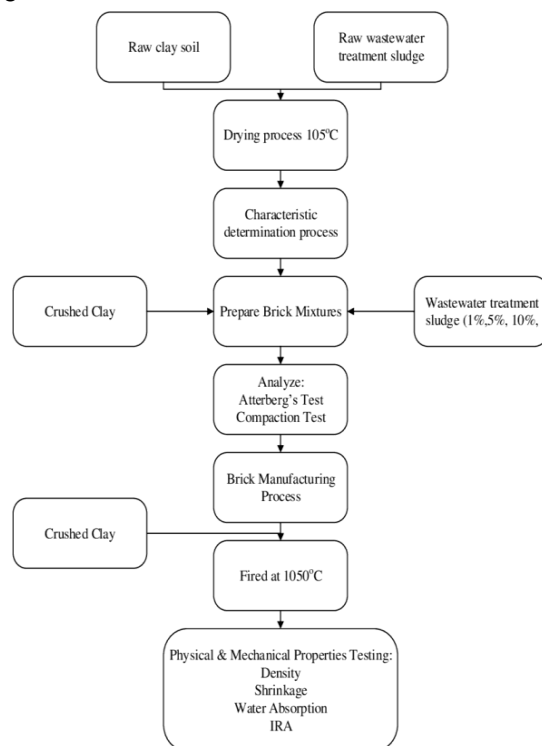
Fig. 1 Flowchart for preparing Brick using Waste Material
