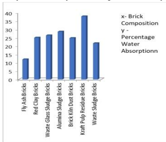
Fig.4 Graph between water absorption and brick composition
