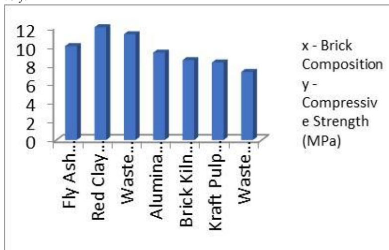
Fig.3 Graph between compressive strength and brick composition
