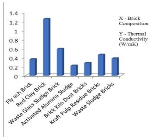
Fig.5 Graph between thermal conductivity and brick composition
