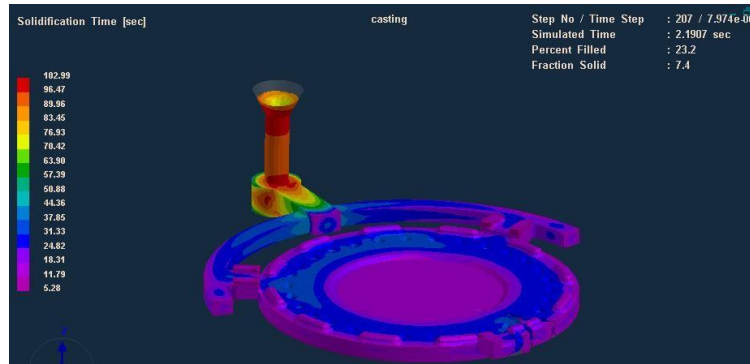
Fig. 5 solidification of molten metal for case I
