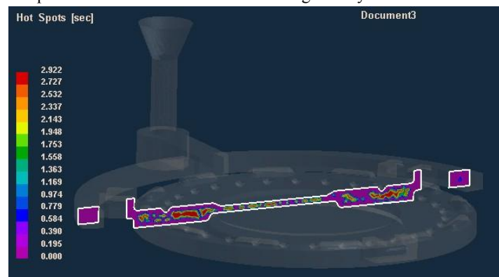
Fig. 6 Hot Spot Zone of casting
