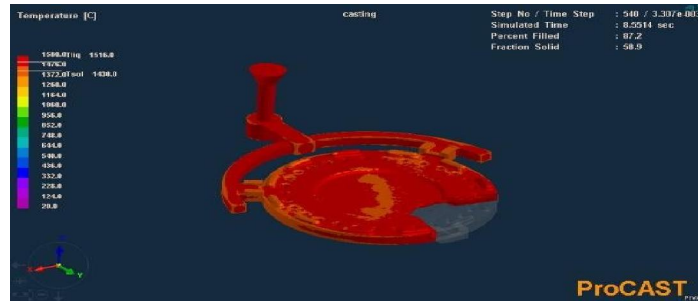
Fig 4 distribution of molten metal into the cavity
