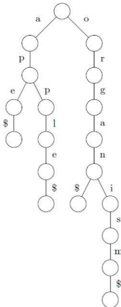
Figure 2: A Trie storing a string
