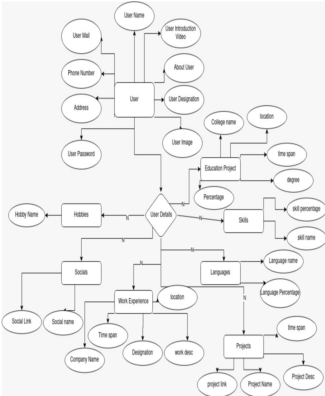
Fig 2: Entity Relationship Diagram
